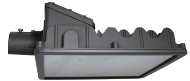
AL35Q Shown with "ALMAA" Pole Mounting Arm Adaptor, Die-Cast Adaptor for 2 3/8" Horizontal Mounting Arms, Bronze Powdercoat Finish, Includes Hardware.
