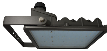
AL35Q Shown with "LFLY" Yoke, Stamped Heavy-Duty Steel Yoke, Bronze Powdercoat Finish, Includes Hardware.
