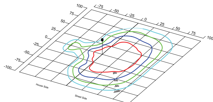
AL35QD1X262U5KC Type IV
