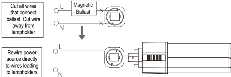
Fig:3 - Magnetic ballast fixture wiring modification (Type B)
