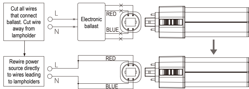
Fig:2 - Electronic ballast fixture wiring (Type B)
