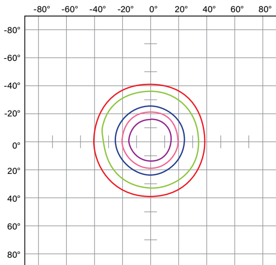
ISOCANDELA PLOT
